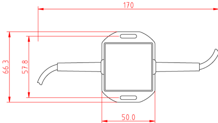
Dimension drawing
