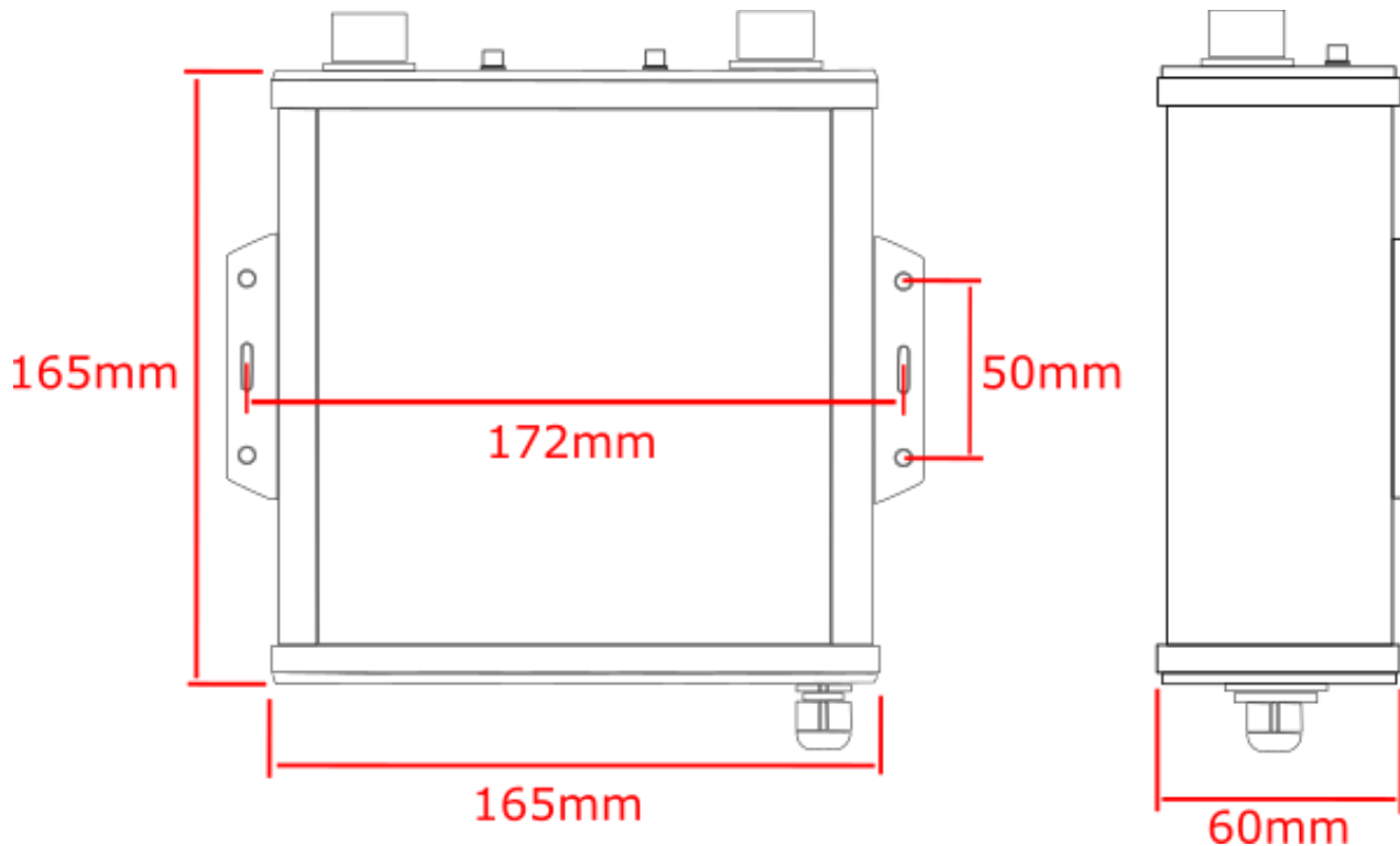
Figure 1 - Dimensions
